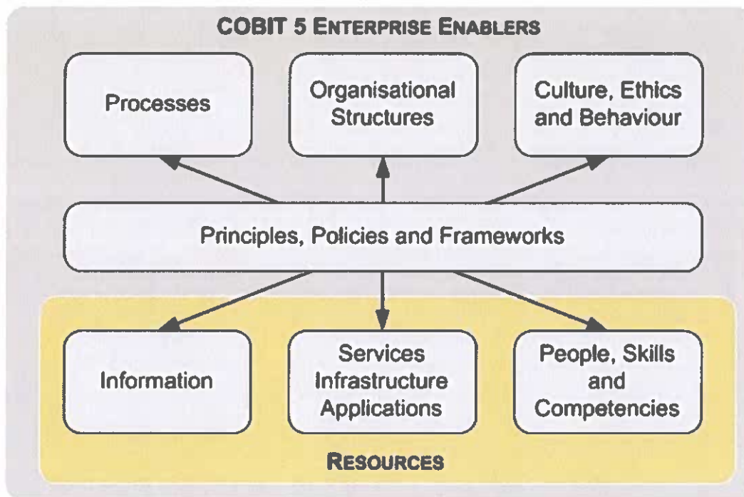
Figure 3: COBIT Enablers
